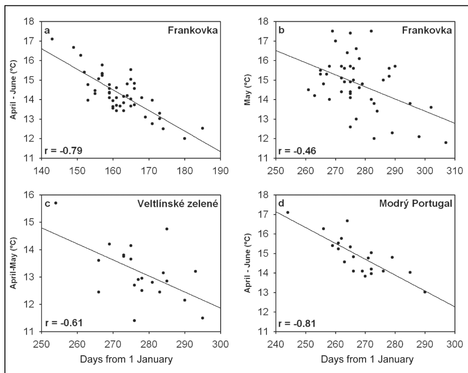
Fig. 6 – Correlations between temperatures and grapevine phenophases for various grape varieties at Velké Pavlovce: a) beginning of flowering, b) beginning of vintage – both 1956–2007, c) and d) beginning of vintage, 1984–2007; r – correlation coefficient.
