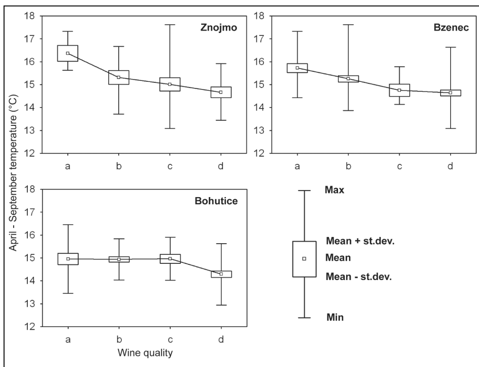
Fig. 5 – Box plot of Brno April–September temperatures calculated for four groups of wine quality in Znojmo (1802–1845), Bzenec (1800–1890) and Bohutice (1861–1912): a – excellent, b – good, c – average, d – bad wine (st. dev. – standard deviation).
