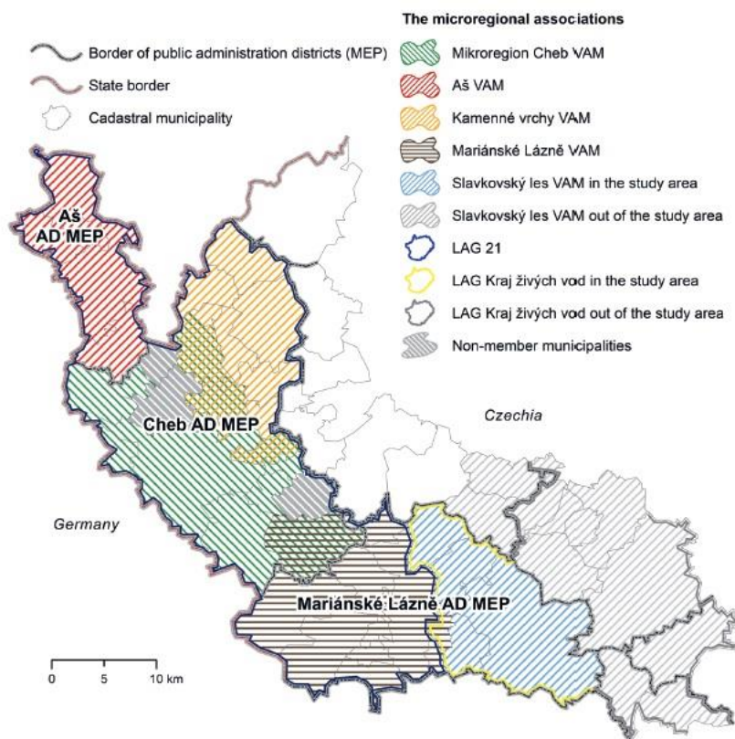
Fig. 4 – Microregional associations in Cheb district in 2020.
